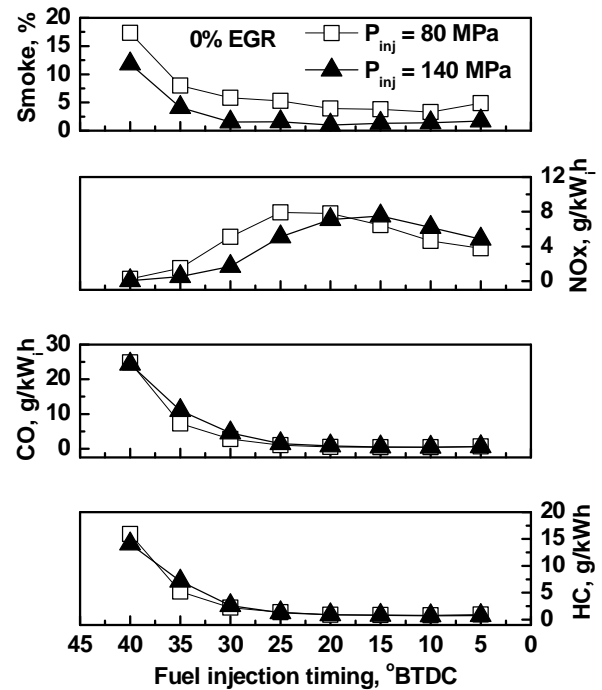
Fig.4. Effect of injection pressure on specific emissions
