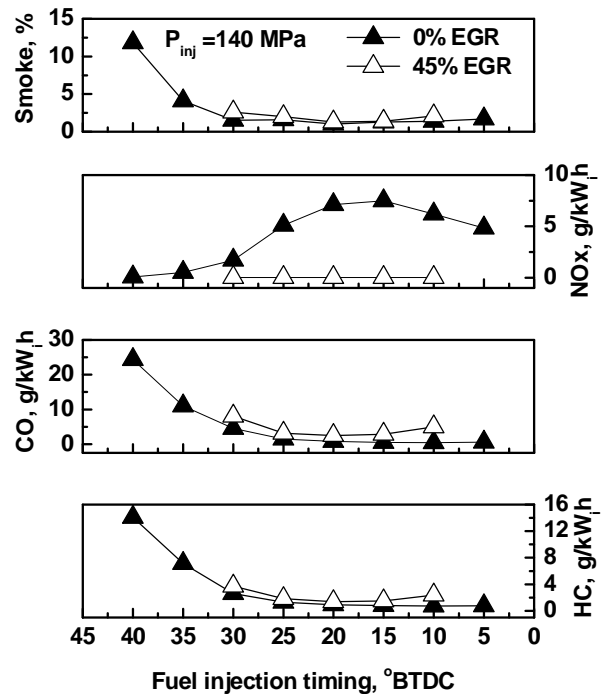
Fig.10. Effect of EGR on specific emissions
