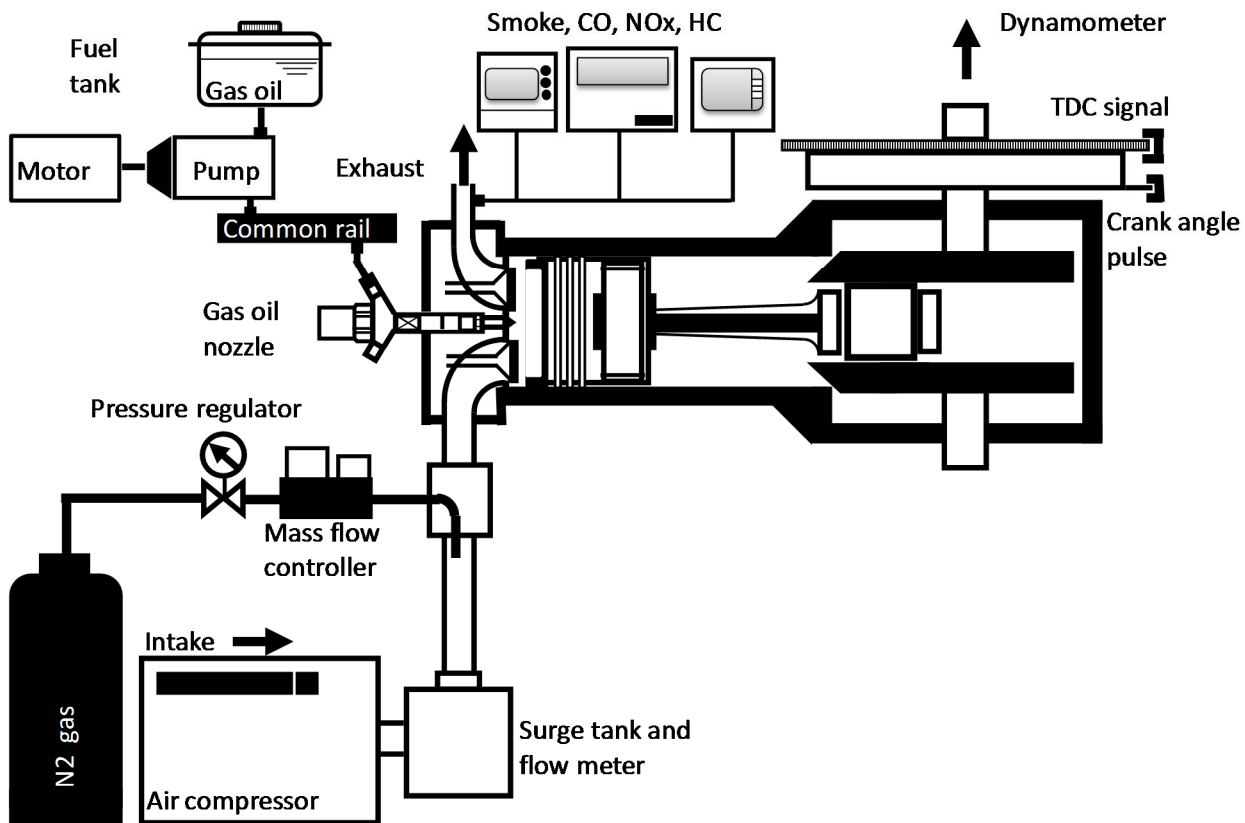
Fig.1. Experimental set up
