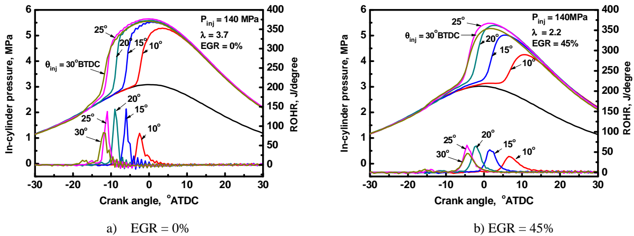
Fig.8. Pressure history and rate of heat release (ROHR) P_{inj} = 140 MPa, \lambda = 3.7 and 2.2 , 0 and 45% EGR
