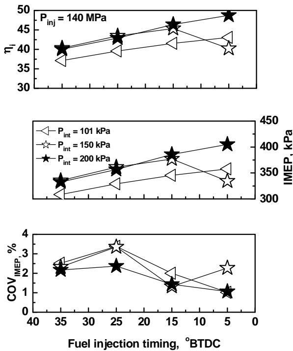
Fig.6. Effect of intake pressure on indicated thermal efficiency, IMEP and COV_{IMEP}
