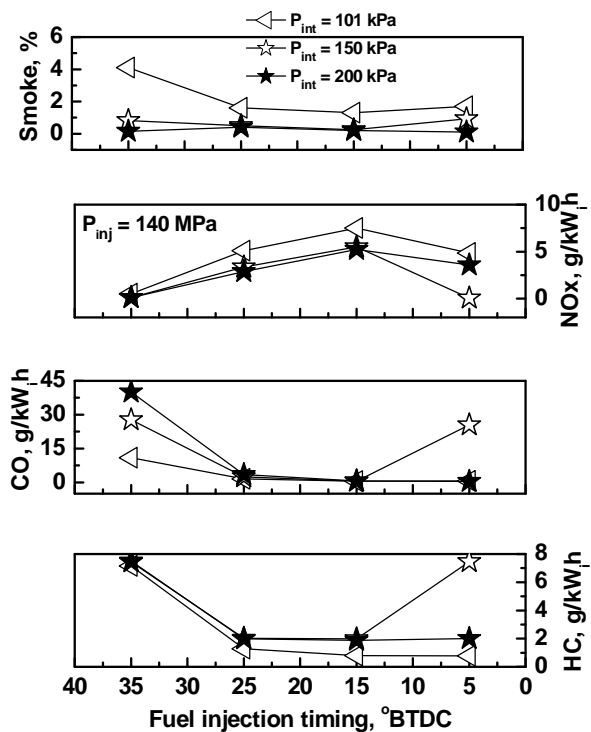
Fig.7. Effect of intake pressure on the specific emissions
