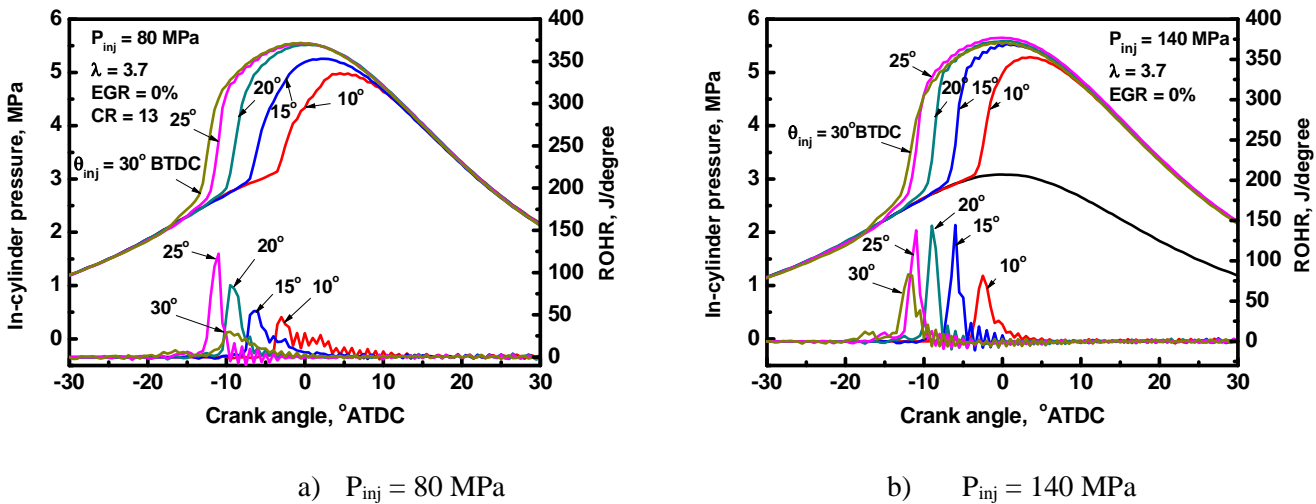
Fig.2. Pressure history and rate of heat release (ROHR) P_{inj} = 80 and 140 MPa, \lambda = 3.7 , 0\% EGR
